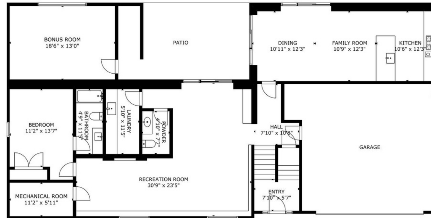
BASEMENT
