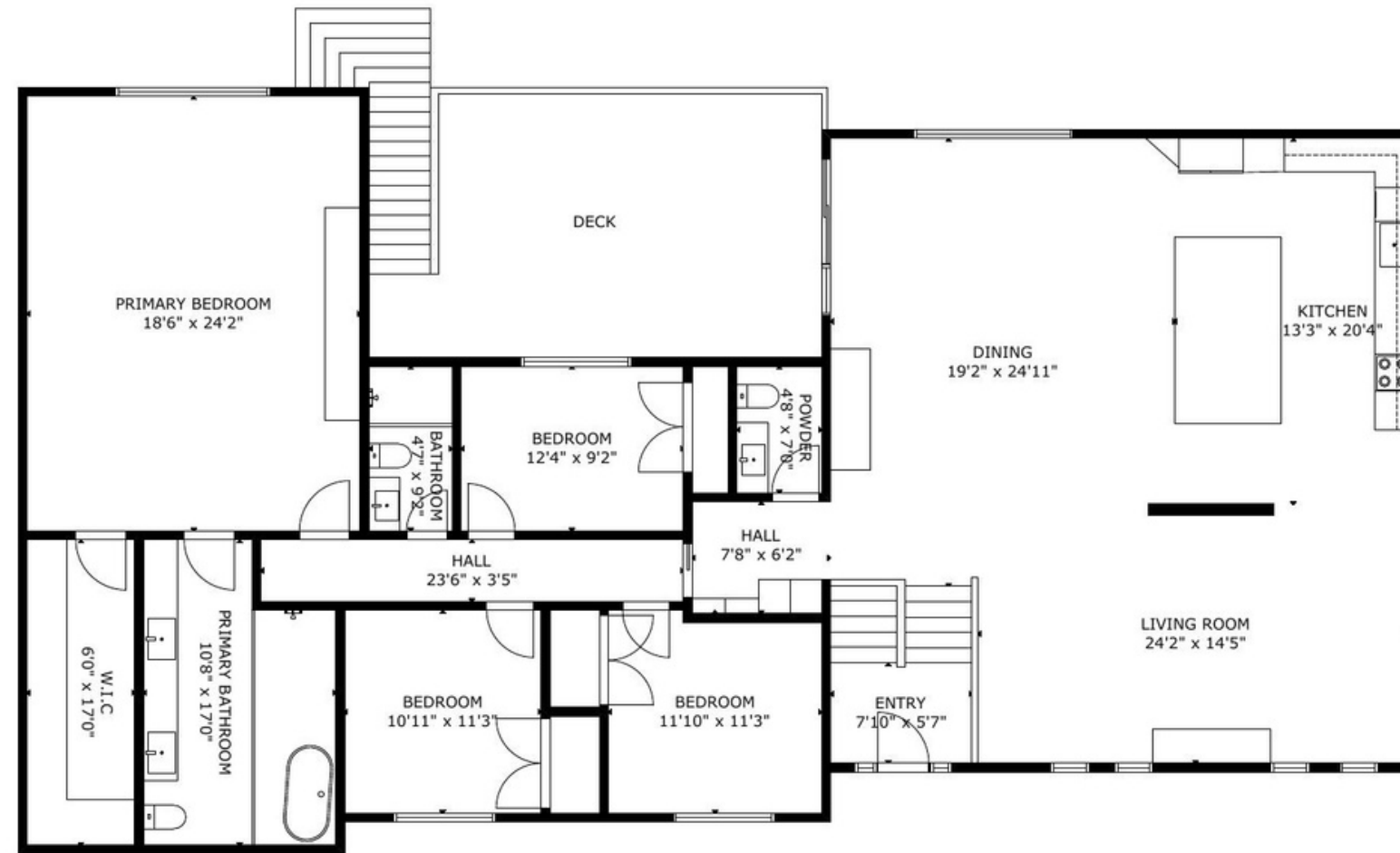
FIRST FLOOR
