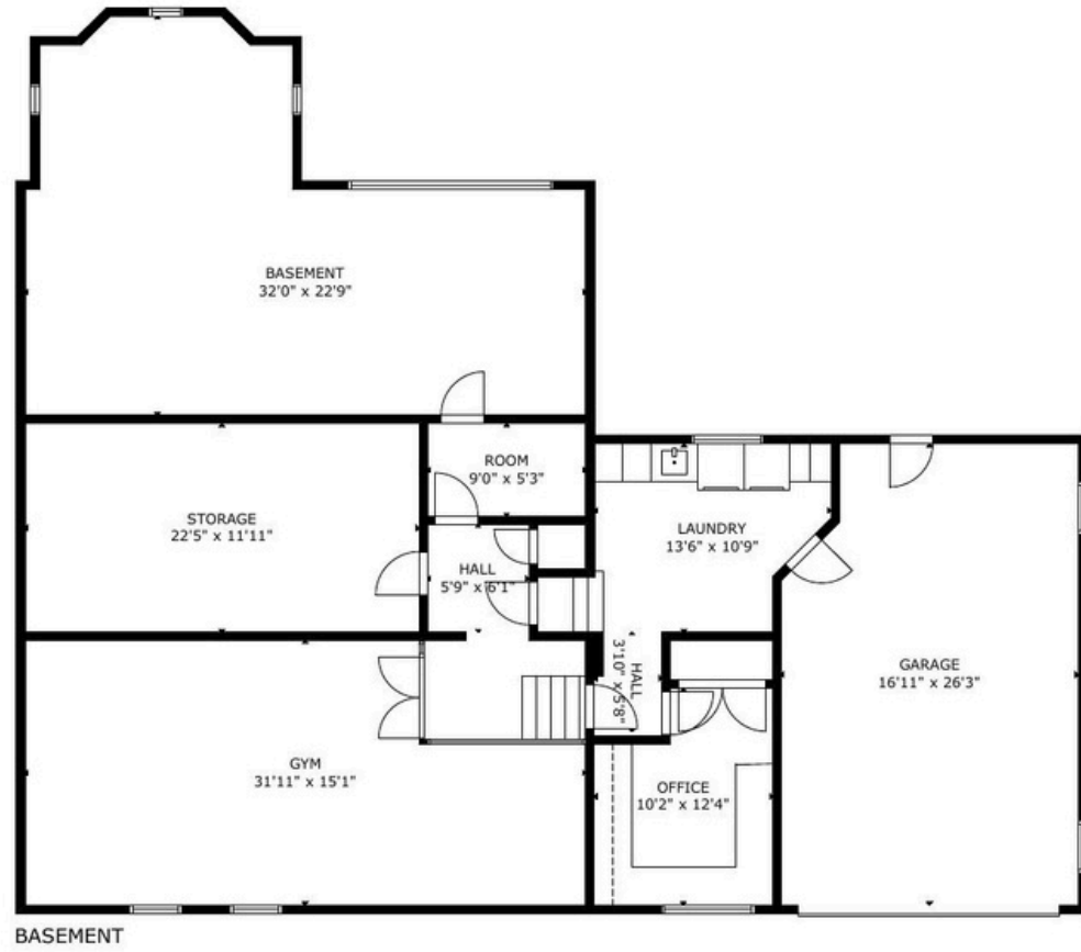
BASEMENT
