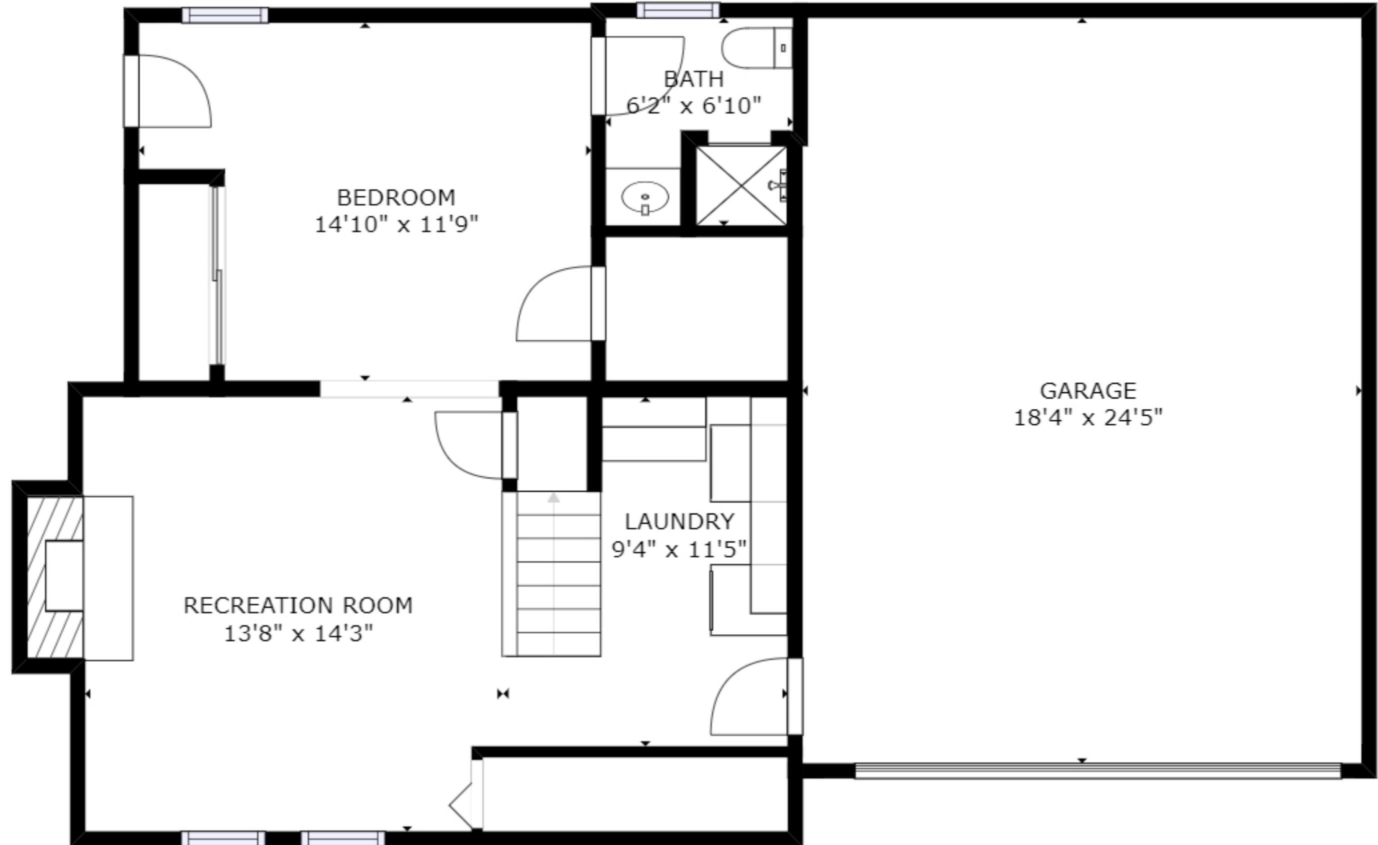
FLOOR 1
